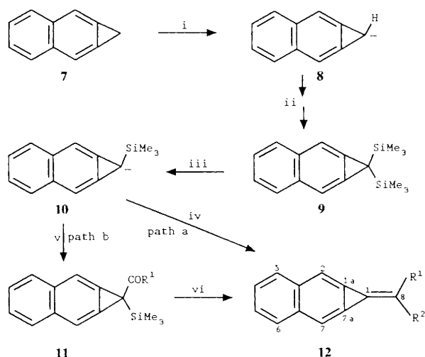
Scheme 2 Reagents and conditions: i. BuLi, THF; ii. \text{Me}_3\text{SiCl} , BuLi, \text{Me}_3\text{SiCl} ; iii. Bu t OK, THF; iv. \text{R}^1\text{R}^2\text{CO} ; v. \text{R}^1\text{COX} ; vi. LiR 2
